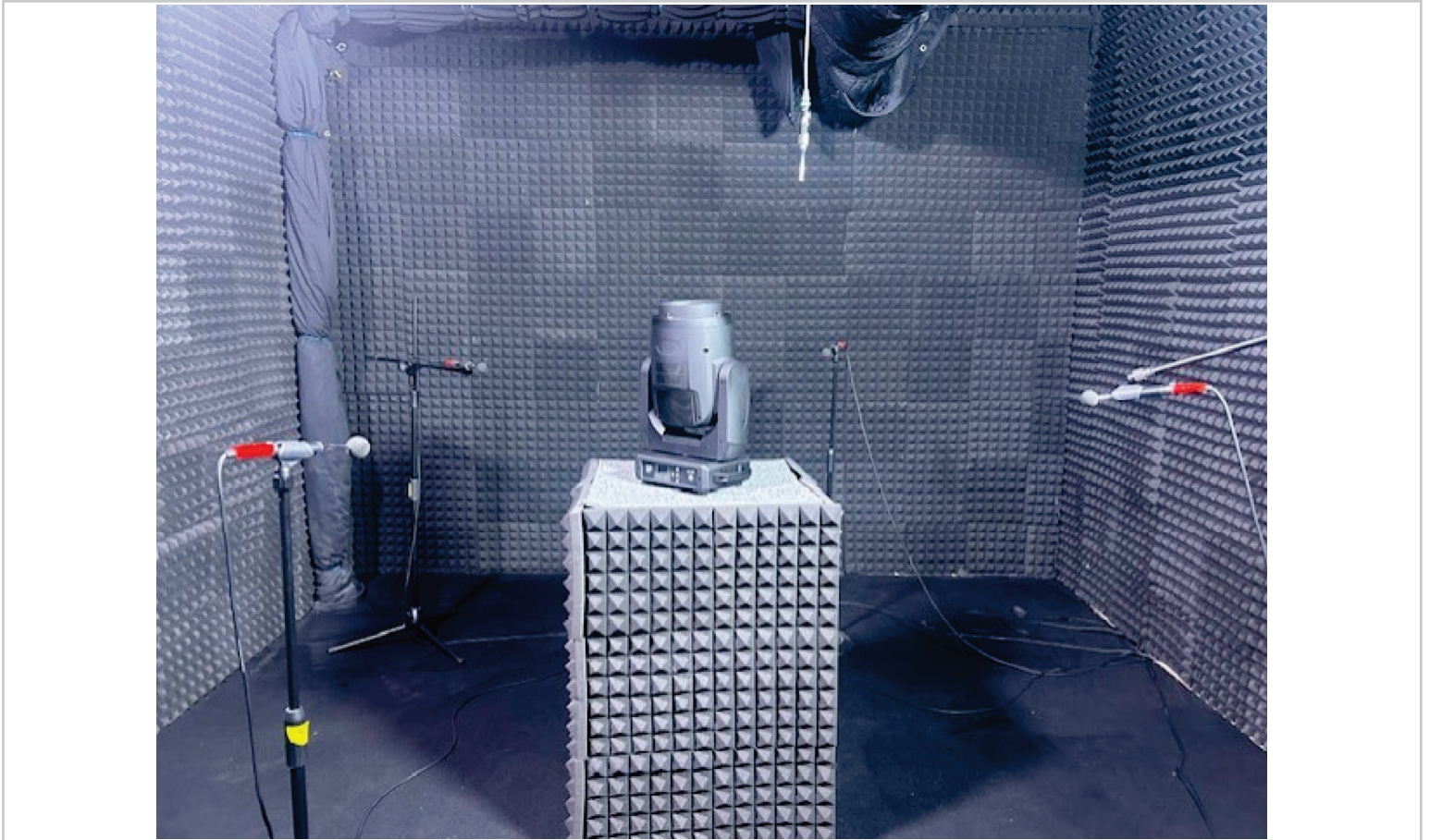
FIGURE 01: TEST SETUP
